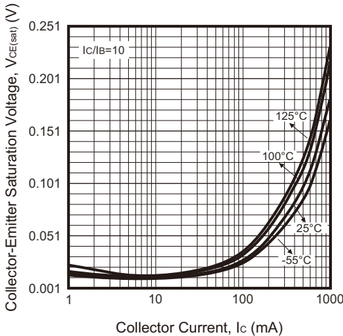
Fig.3 - V_{CE(sat)} — I_C
