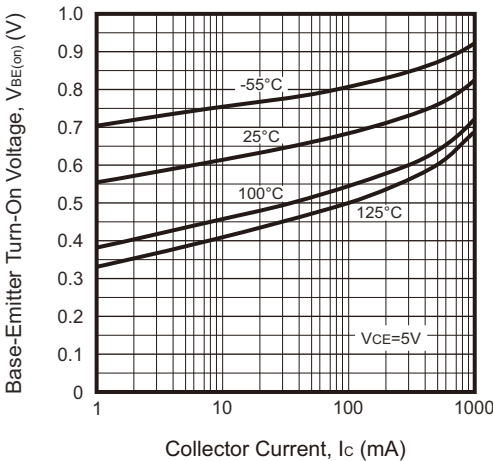
Fig.4 - V_{BE(on)} — I_C
